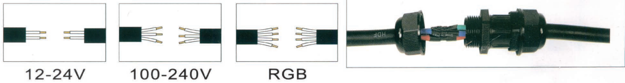
Wiring Diagram
