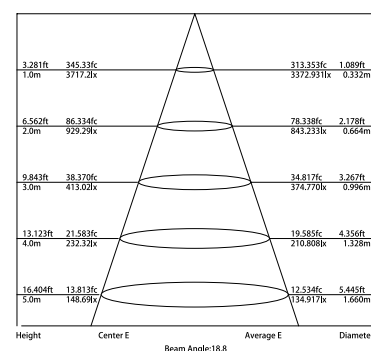
Lux distance Curve
