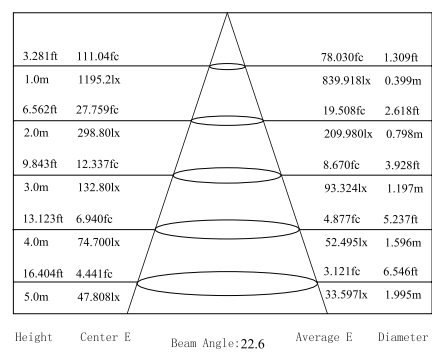
Lux distance Curve
