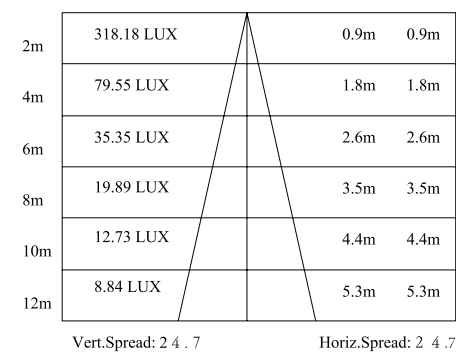
Lux distance Curve
