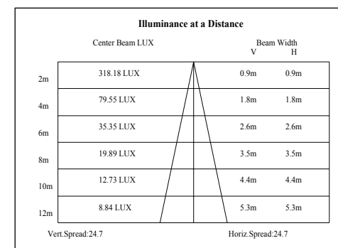
Lux distance Curve
