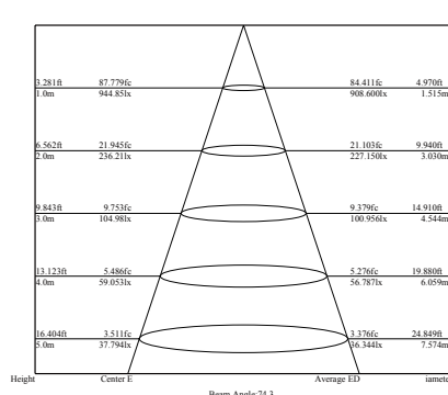
Lux distance Curve
