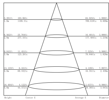
Lux distance Curve
