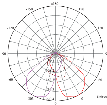
Light Distribution Curve [Unit: cd]
